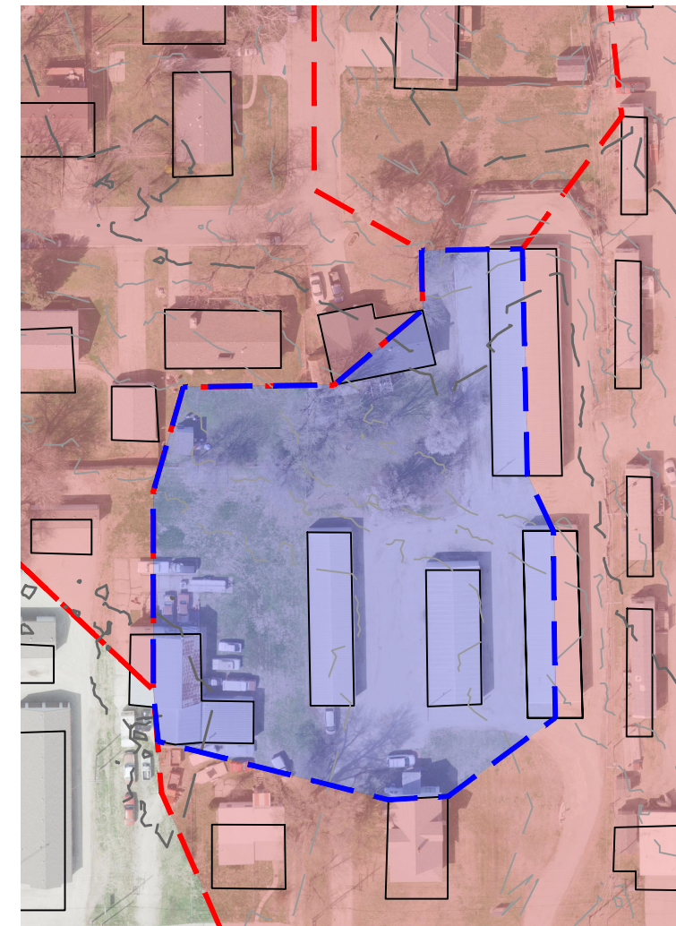
PROPOSED DRAINAGE BASIN "A" MAP Scale: 1"=100'
